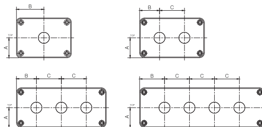
PUSH BUTTON HOLE SPACING
